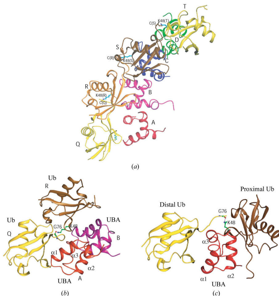
Figure 7 A model for tetraubiquitin (Ub 4 ) binding to four Dsk2 UBA molecules. (a) The Dsk2 UBA molecules, arranged in a ninefold helix as in the UBA/UBL crystal structure, are labelled A, B, C and D and coloured red, magenta, blue and green, respectively. The Ub 4 subunits, modelled on the UBL structure in the UBA–UBL complex, are labelled Q, R, S, T and colored yellow, orange, brown and yellow, respectively. They are linked by an isopeptide bond from the C-terminal G76 of one Ub molecule to K48 (shown in cyan) of the neighboring Ub molecule. (b) An enlarged view of the Dsk2 UBA dimer associated with the modelled Ub 2 showing the C-terminal G76–K48 linker. (c) The HR23A UBA–Ub 2 complex from Varadan et al. (2005) with the distal Ub molecule oriented as in the Ub molecule Q in (b). The diagram illustrates the different modes of association of the different UBA domains and the flexibility of the G76–K48 linker.
