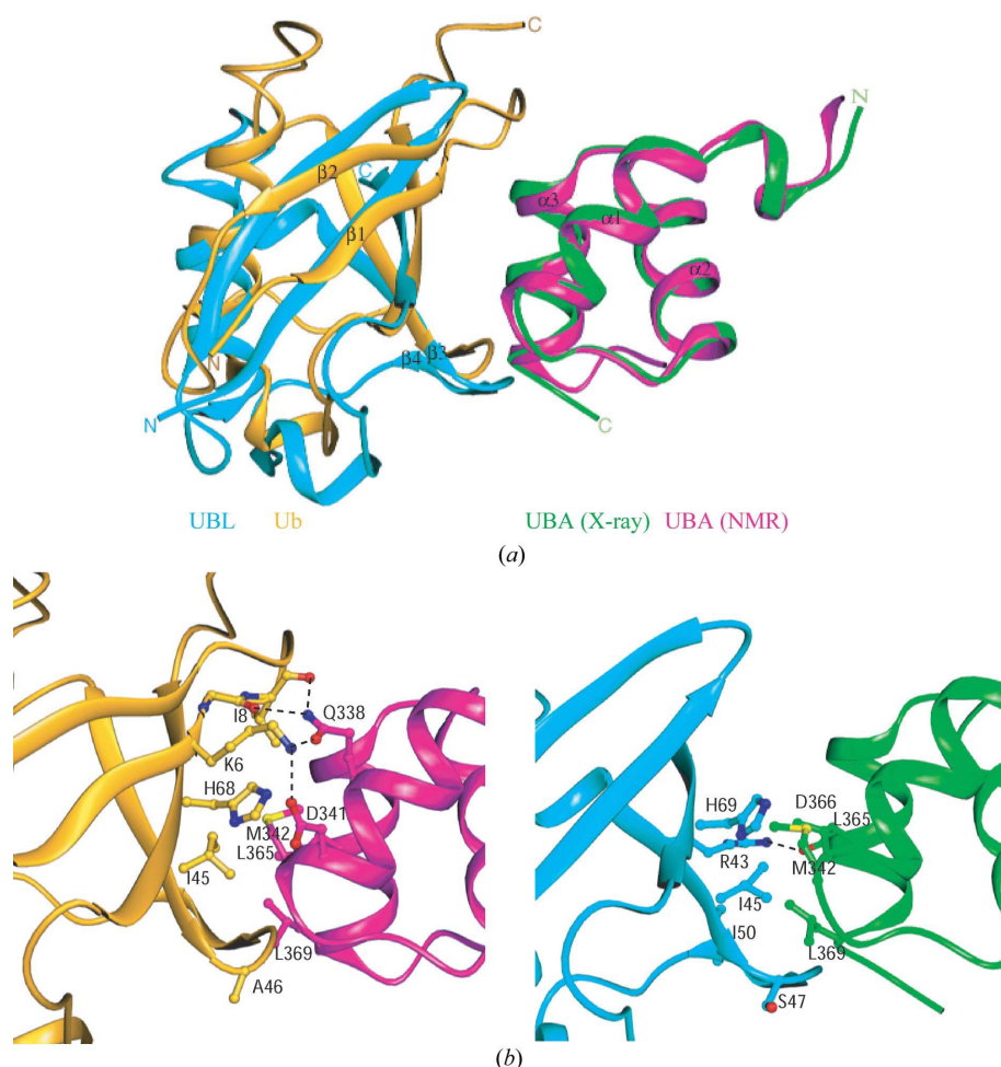
Figure 6 ( a ) Comparison of the Dsk2 UBA–UBL complex (green and cyan, respectively) with the Dsk2 UBA–Ub complex (magenta and orange, respectively; from Ohno et al. , 2005). The major differences at the interface are at the \beta 1/\beta 2 loop and the \beta 3/\beta 4 loop of UBL and Ub. Further details are described in the text. ( b ) A simplified view of the contacts between Ub (gold) and UBA (magenta) (left) and UBL (cyan) and UBA (green) (right) showing the domains in the same orientation as Fig. 6( a ). Only the most significant contacts that differ between the two structures are shown. The Ub–UBA interface has contacts from Ub residues K6 and L8 to UBA residues which are not made in the UBL–UBA complex. The UBL–UBA complex has closer contacts between I45 and I50 with UBA residues L365 and L369 than in the Ub–UBA complex. Full details of the contacts are given in the supplementary material.
